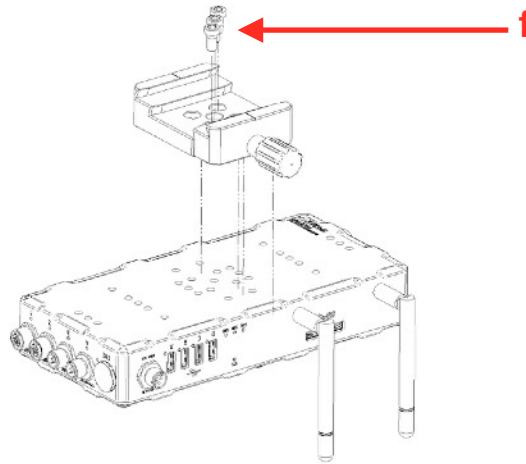
Image 35: installation of "Vixen+Losmandy PLUS dovetail clamp" on EAGLE
